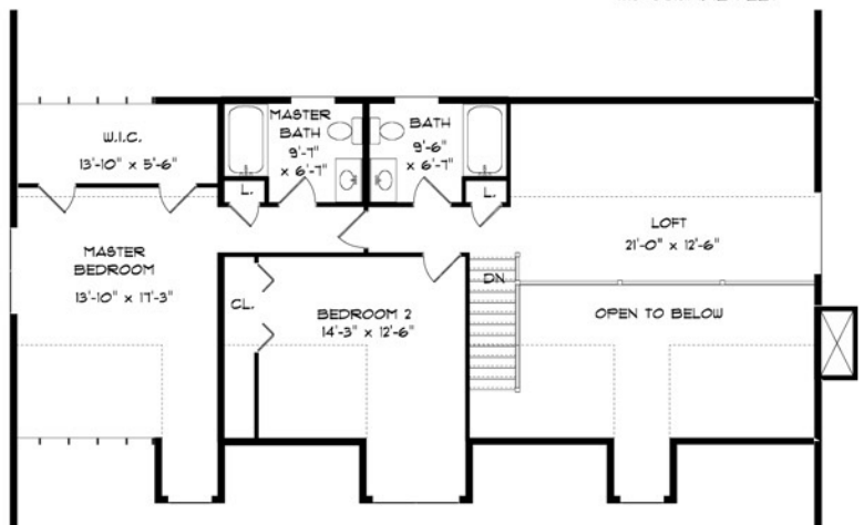
SECOND FLOOR 1115 SQUARE FEET
